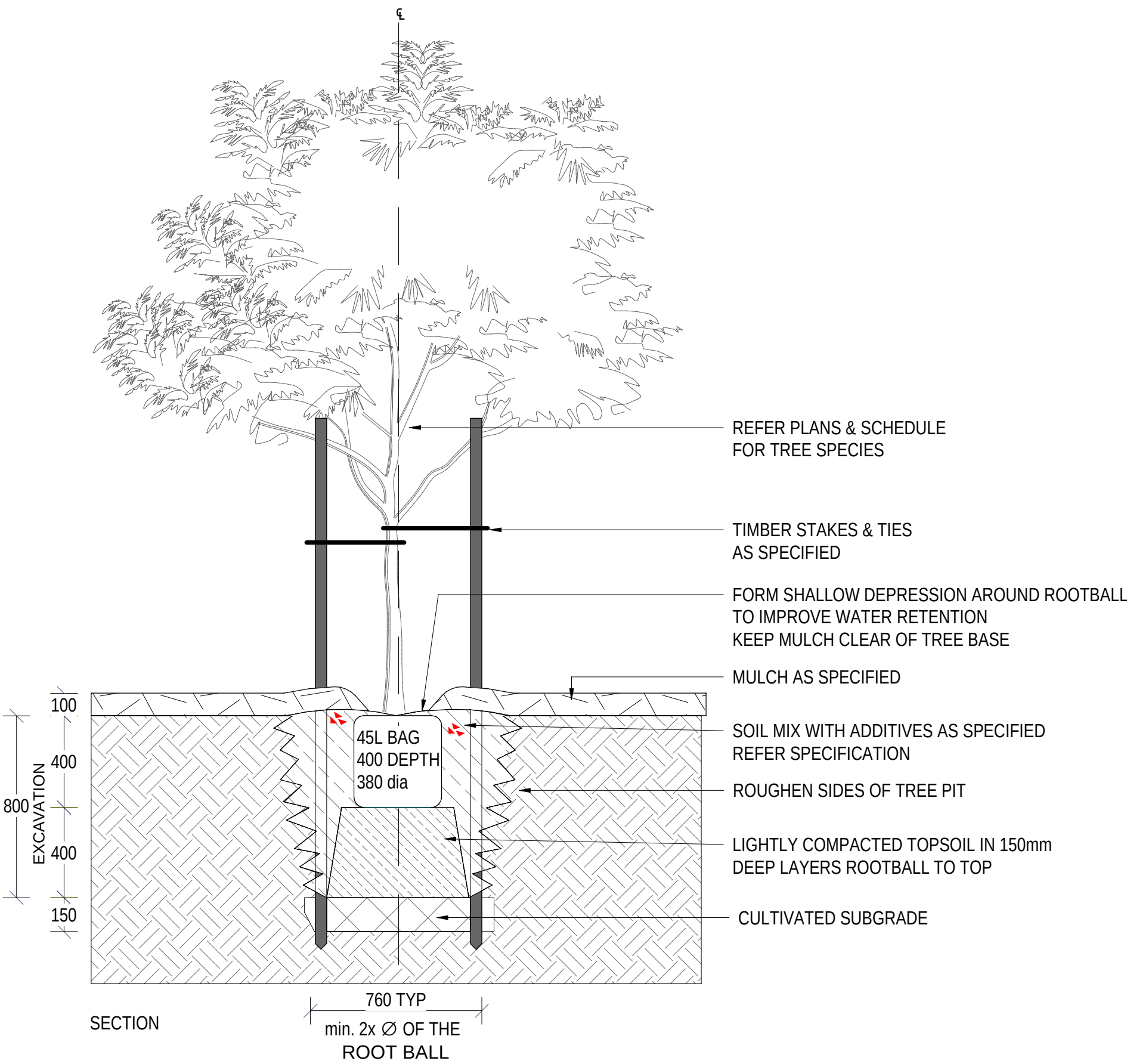
1 45L TREE IN PLANTING IN NATURAL GROUND SCALE - 1 : 20
