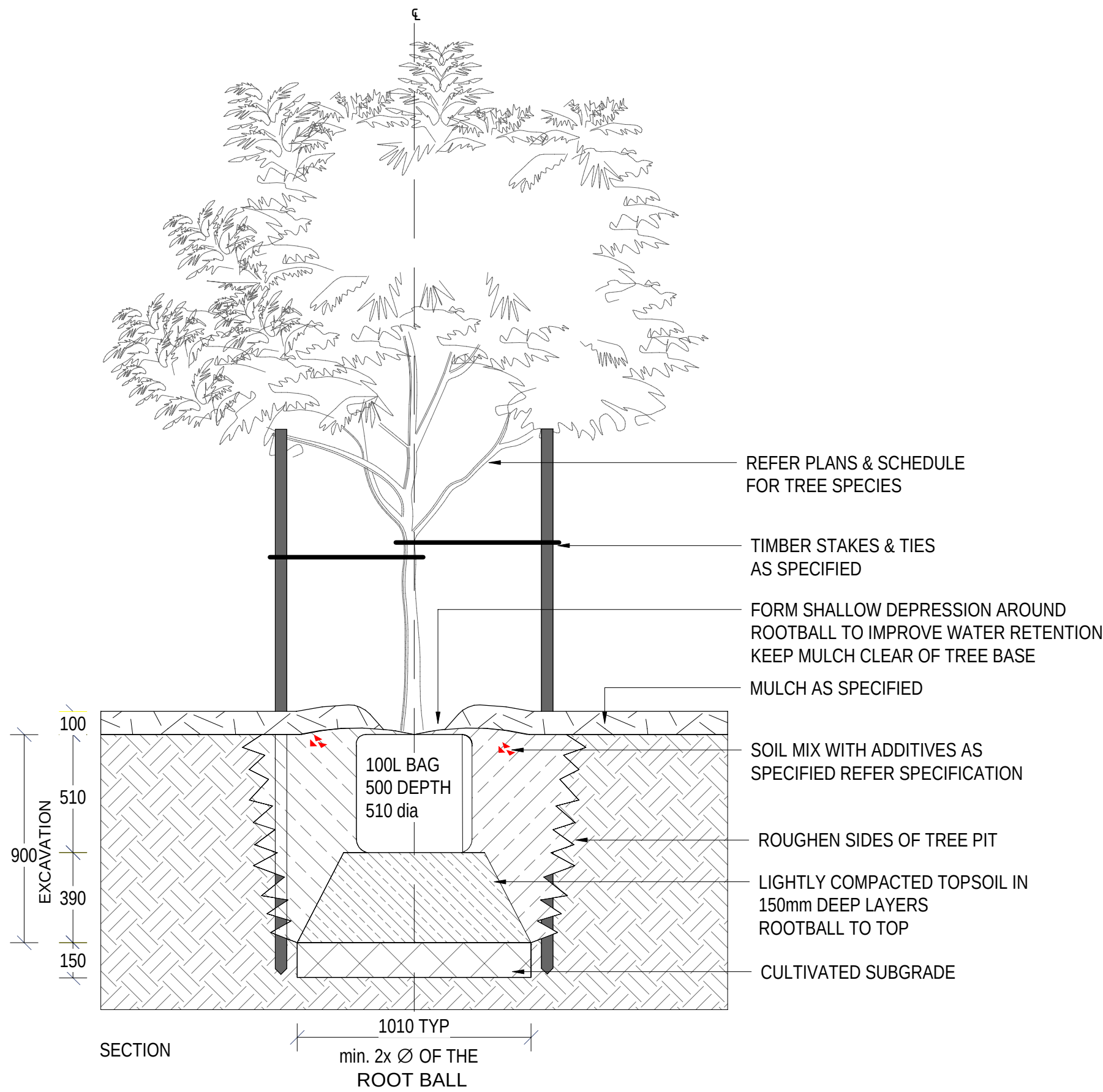
2 100L TREE IN PLANTING IN NATURAL GROUND SCALE - 1 : 20
